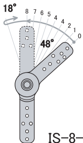
IS-8-132 zero position= 132° end position= 180°
