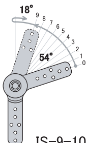
IS-9-108 zero position= 108° end position= 162°
